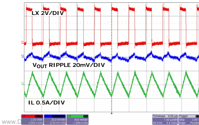
FIGURE 17. STEADY STATE OPERATION AT NO LOAD (PWM)
